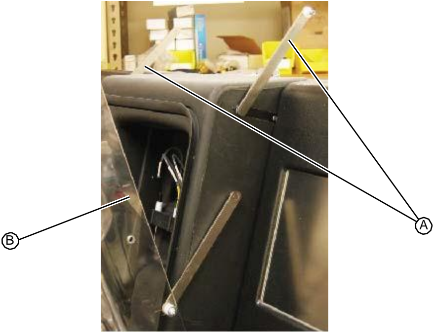
Figure 8.9: Vacuum chamber door hinge arm
