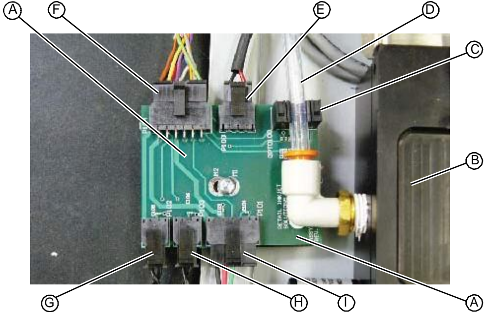
Figure 8.36: Fluid sensor board connections
