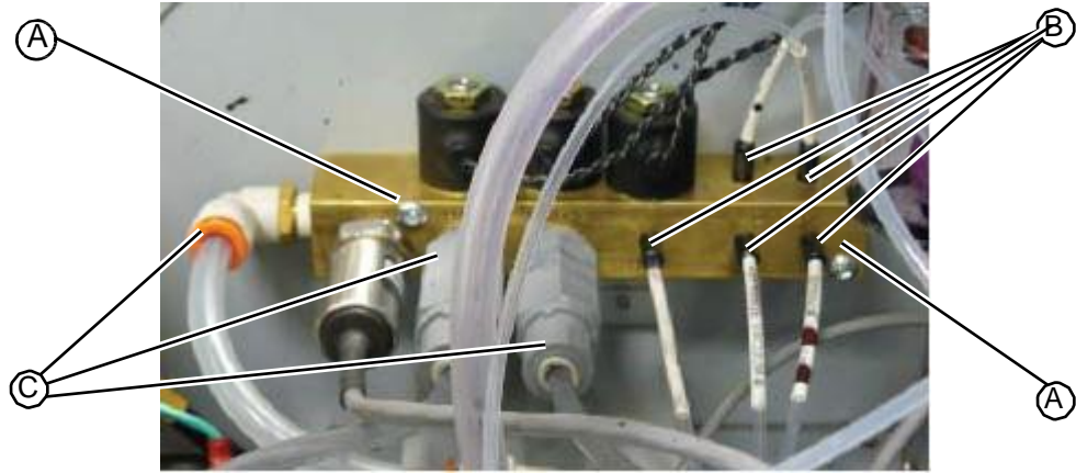
Figure 8.48: Vacuum distribution manifold
