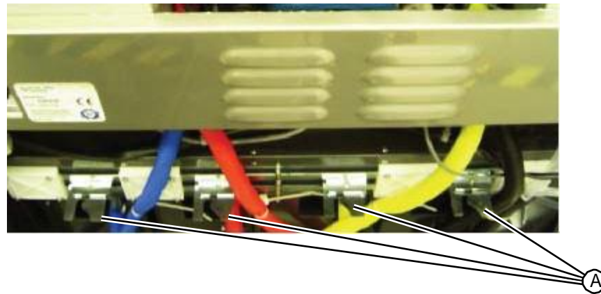
Figure 8.52: Interlock guide plates cover
