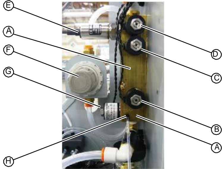
Figure 8.46: Main vacuum manifold
