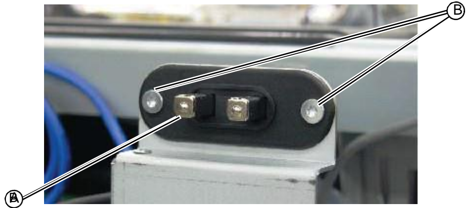
Figure 8.51: Upper hood fan power contacts
