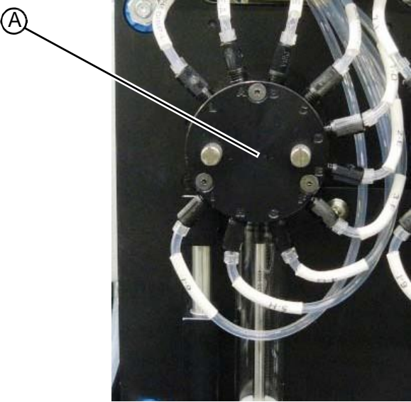
Figure 8.20: Fluid distribution valve
