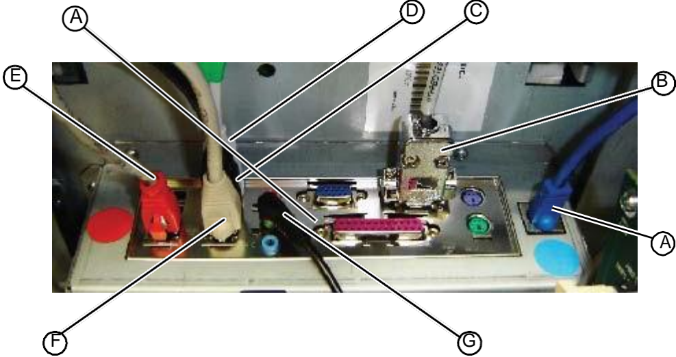
Figure 8.34: Cable connections on top of the touchscreen assembly
