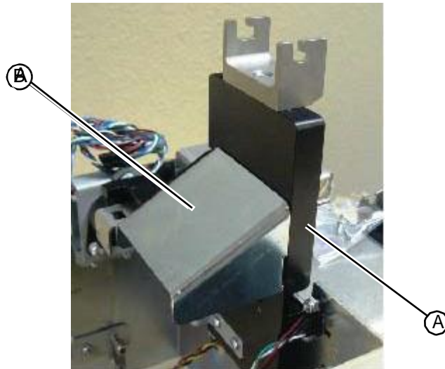
Figure 8.25: Tester cover fixture
