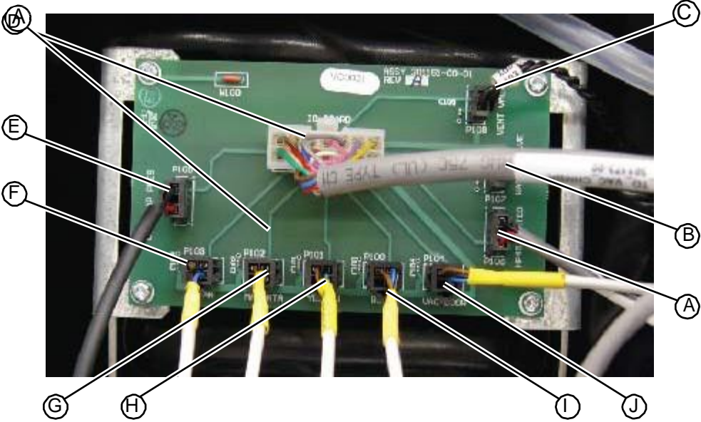
Figure 8.35: Cable connections on the vacuum chamber PC board
