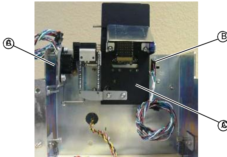
Figure 8.26: Location of the thru-beam paper sensors from the back of the tester assembly
