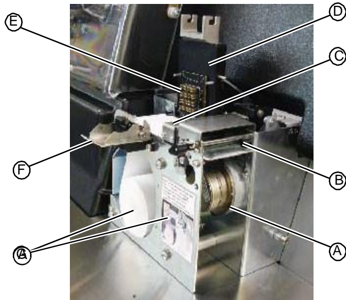
Figure 8.22: Tester station assembly with tester cover removed
