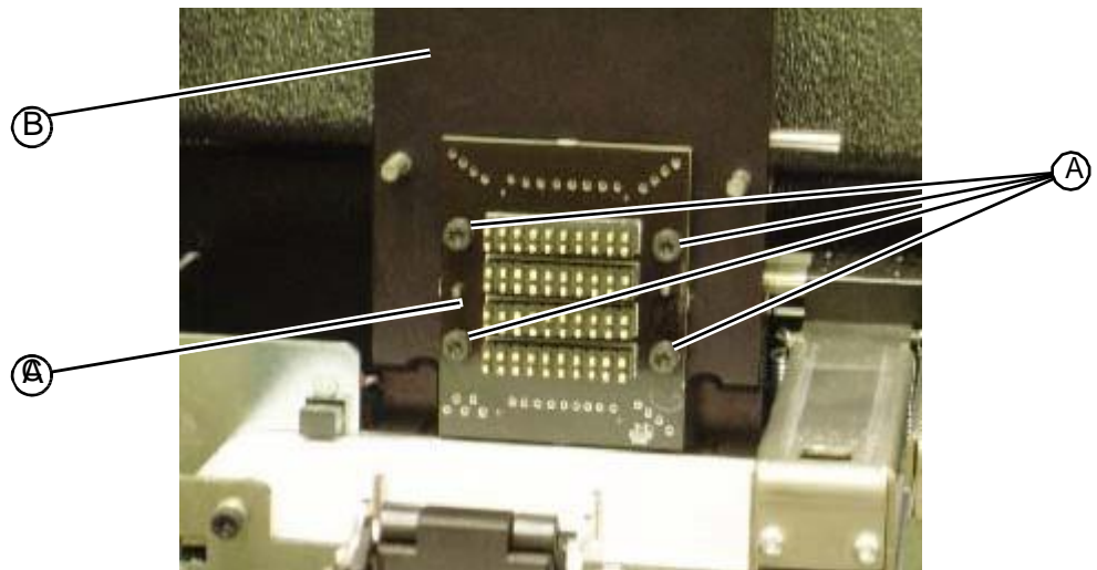
Figure 8.27: Tester interconnect board
