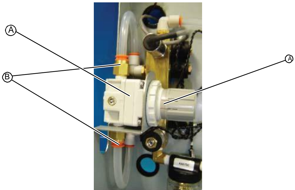
Figure 8.47: Vacuum regulator assembly
