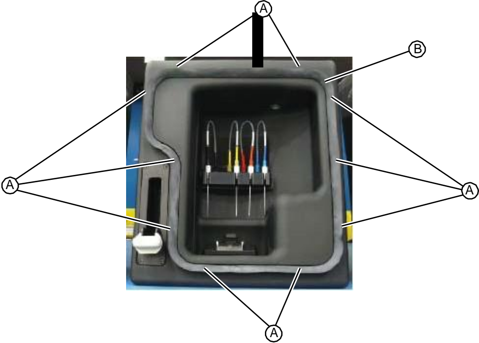
Figure 8.13: Vacuum gasket
