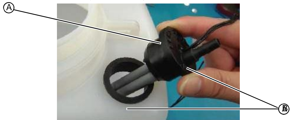
Figure 8.43: Level switch/siphon assembly
