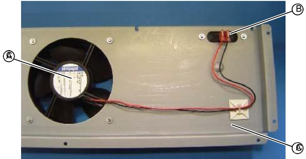
Figure 8.50: Upper hood fan and stationary side spring contacts
