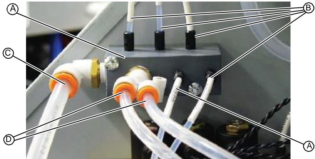
Figure 8.40: Fluid distribution manifold
