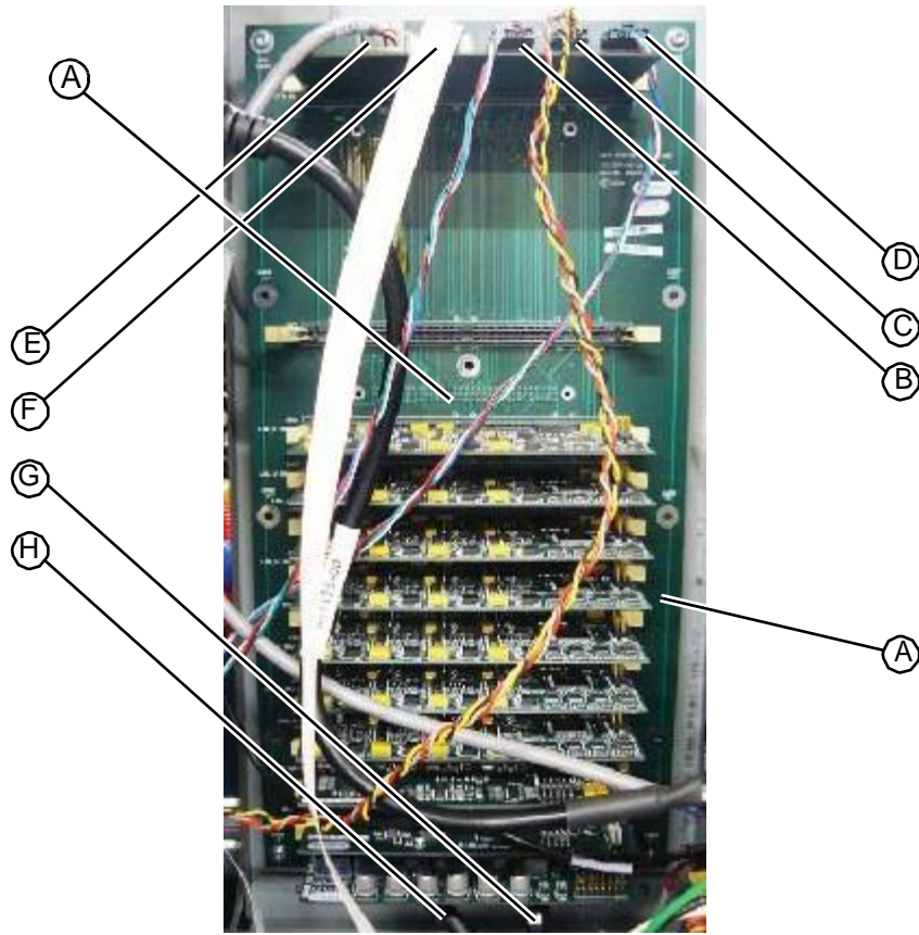
Figure 8.37: Cable connections at the tester PC backplane board.
